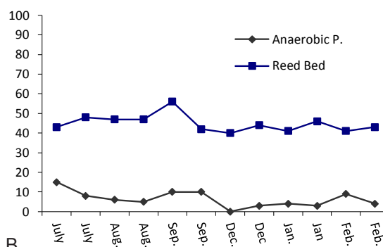
Figure 4. (A) Average TN removal; and (B) average TP removal in reed beds and anaerobic ponds for total study period.
