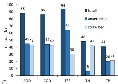
Figure 3. Average parameter removal in anaerobic ponds and reed beds in (A) hot months; (B) cold months; and (C) overall.
